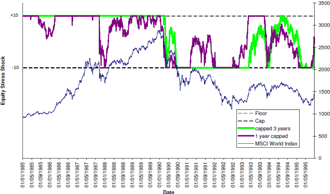
Figure 7: symmetric adjustment comparing 1 and 3 year moving averages 107
